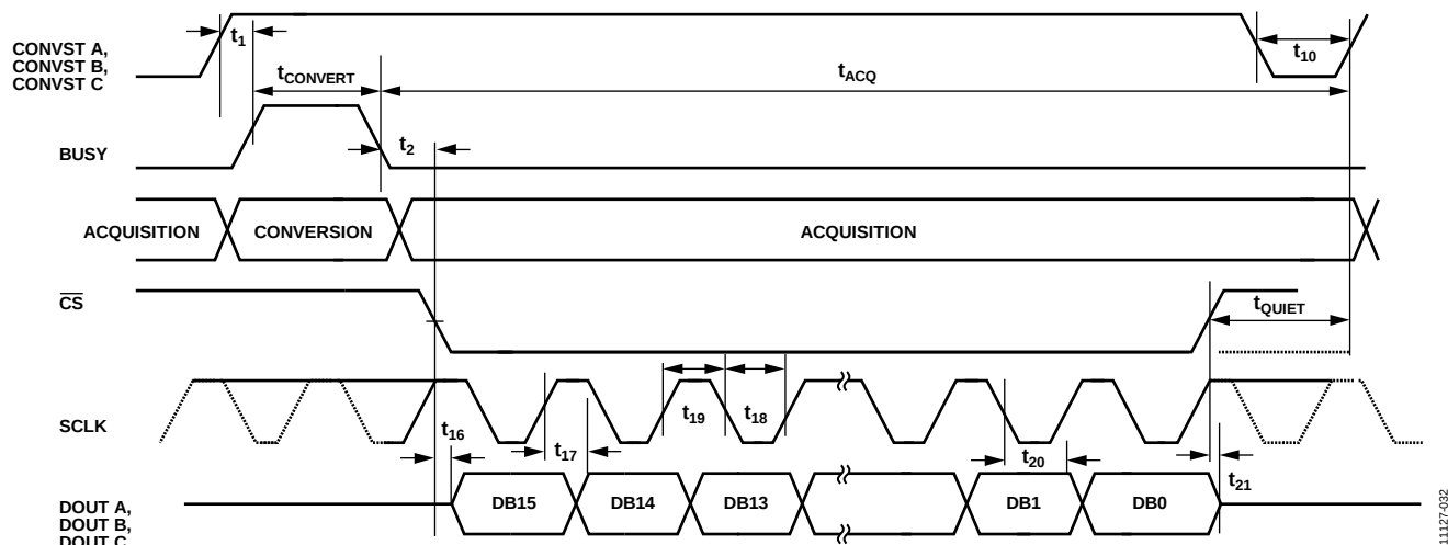
Figure 28. Serial Read Operation
