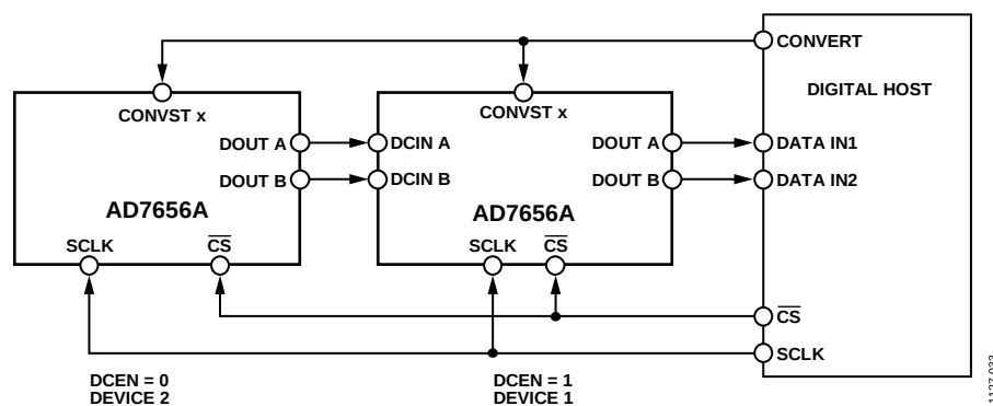
Figure 29. Daisy-Chain Configuration
