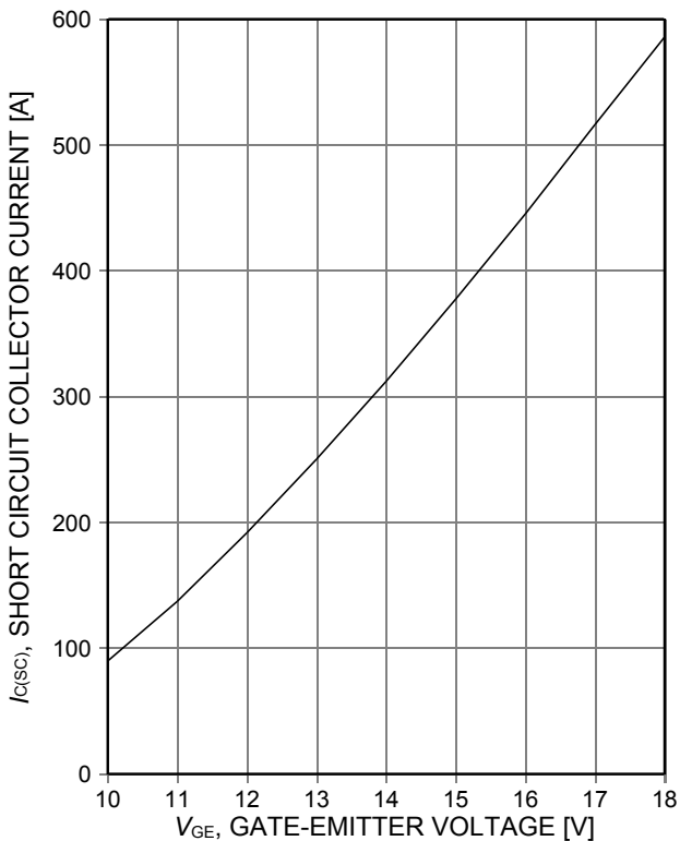
Figure 18. Typical short circuit collector current as a function of gate-emitter voltage ( V_{CE}\leq 600 V, T_{vj}\leq 175^\circ\text{C} )
