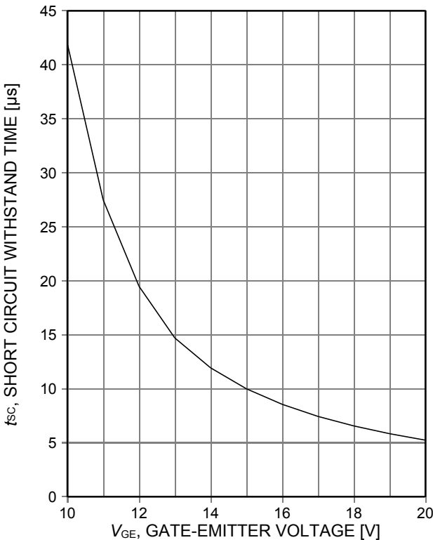
Figure 19. Short circuit withstand time as a function of gate-emitter voltage ( V_{CE}\leq 600 V, start at T_{vj}\leq 175^\circ\text{C} )
