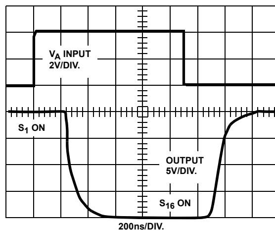
FIGURE 6D. WAVEFORMS
