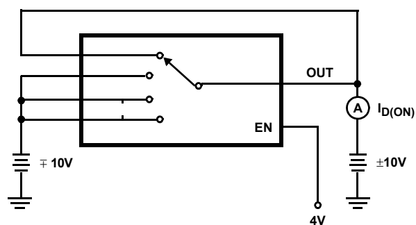
FIGURE 2D. I_{\text{D(ON)}} TEST CIRCUIT (NOTE 9)
