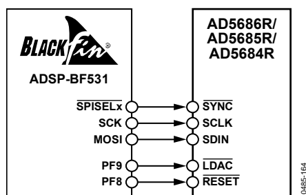
Figure 59. ADSP-BF531 Interface
