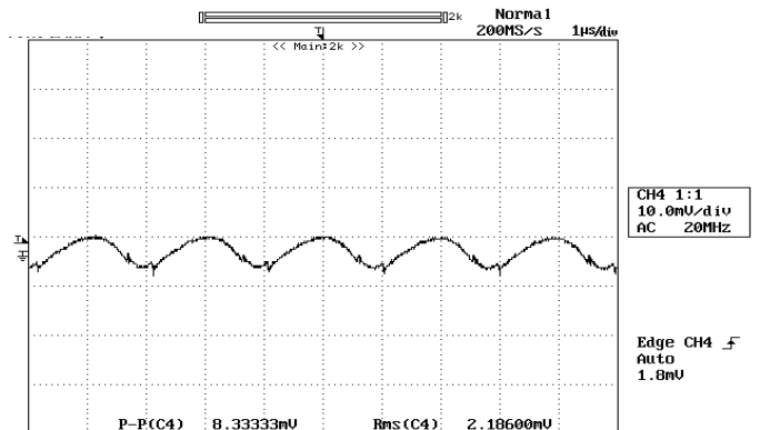
Figure 10: Output ripple & noise at 12Vin, 2.5V/20A out
