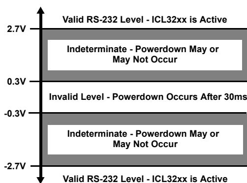
Figure 12. Definition of Valid RS-232 Receiver Levels
