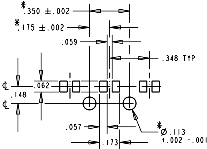
SOLDER PAD/HOLES LAYOUT (SINGLE COLOR SMT LEDS SHOWN)
