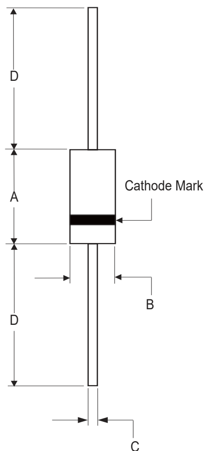
DO-201AE
