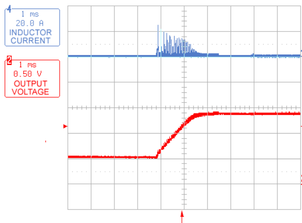
FIGURE 9. PREBIASED START-UP IN DCM MODE
