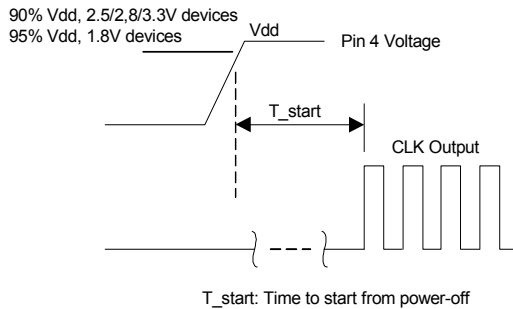
(ST/OE Mode)
