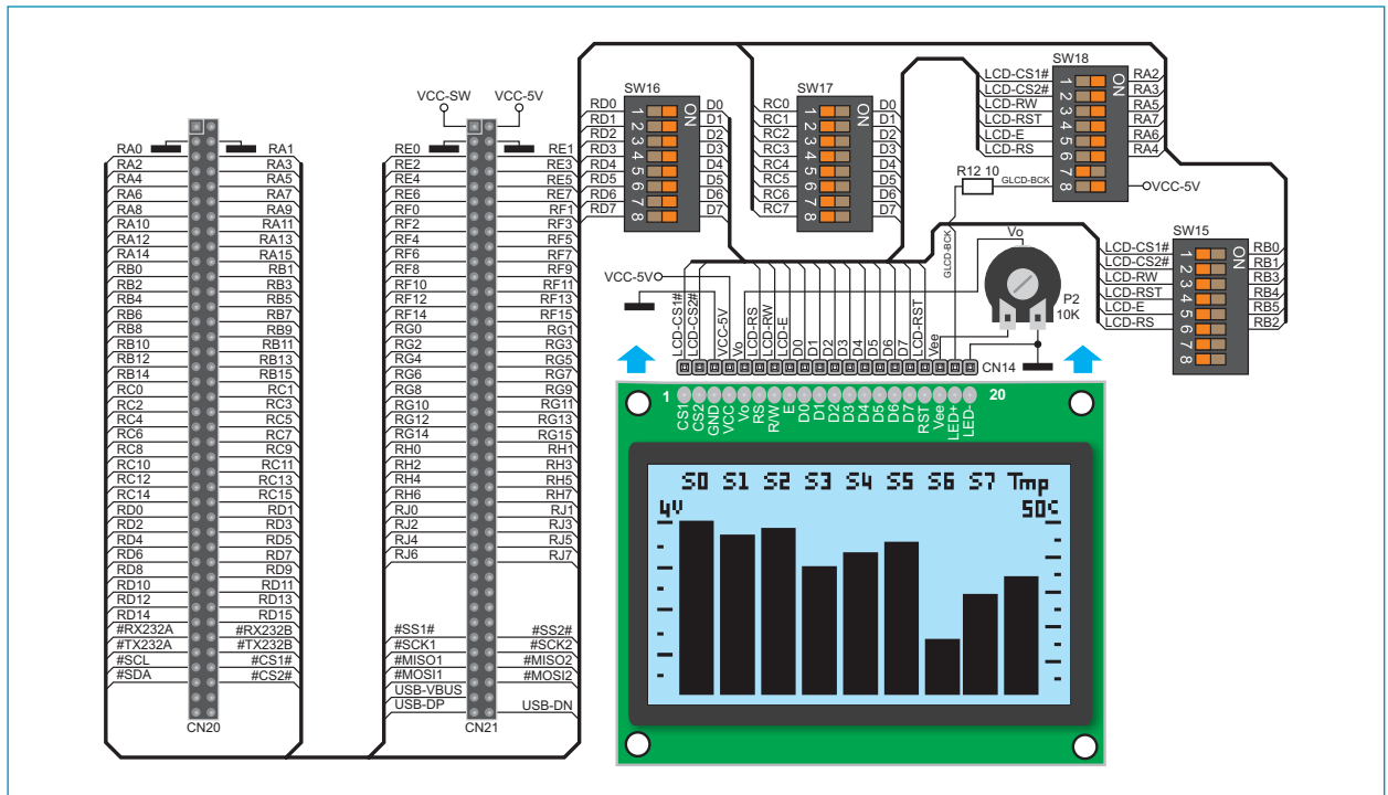
Figure 15-1: GLCD display
