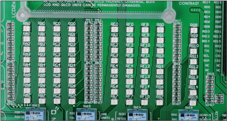
Figure 12-1: LEDs
