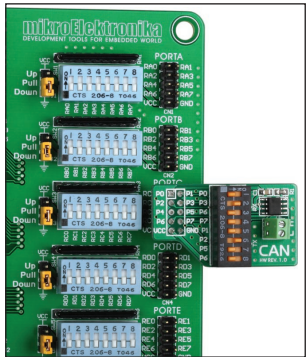
Figure 17-2: Additional board connected to I/O port
