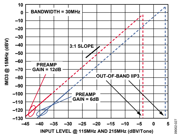
Figure 27. Out-of-Band IIP3: IMD3 Tone at Midband (Bandwidth Setting = 30 MHz)
