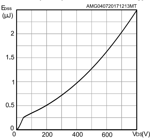
Figure 13: Output capacitance stored energy
