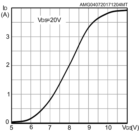
Figure 9: Transfer characteristics
