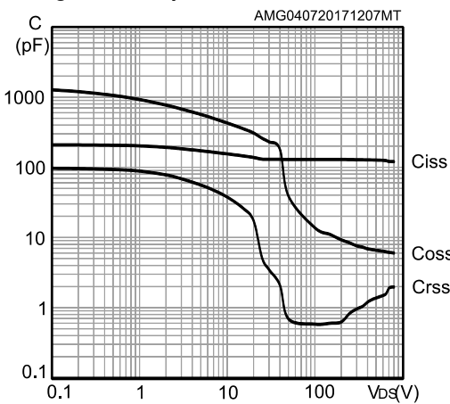
Figure 12: Capacitance variations
