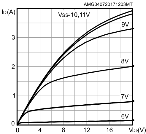
Figure 8: Output characteristics
