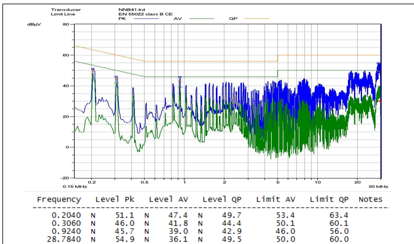
Figure 28 Conducted emissions at 230 V AC neutral and 33 W load - &gt; 7 dB margin
