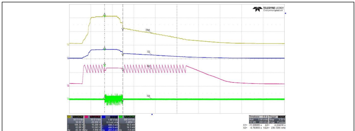
Figure 22 Brown-in/Brown-out protection
