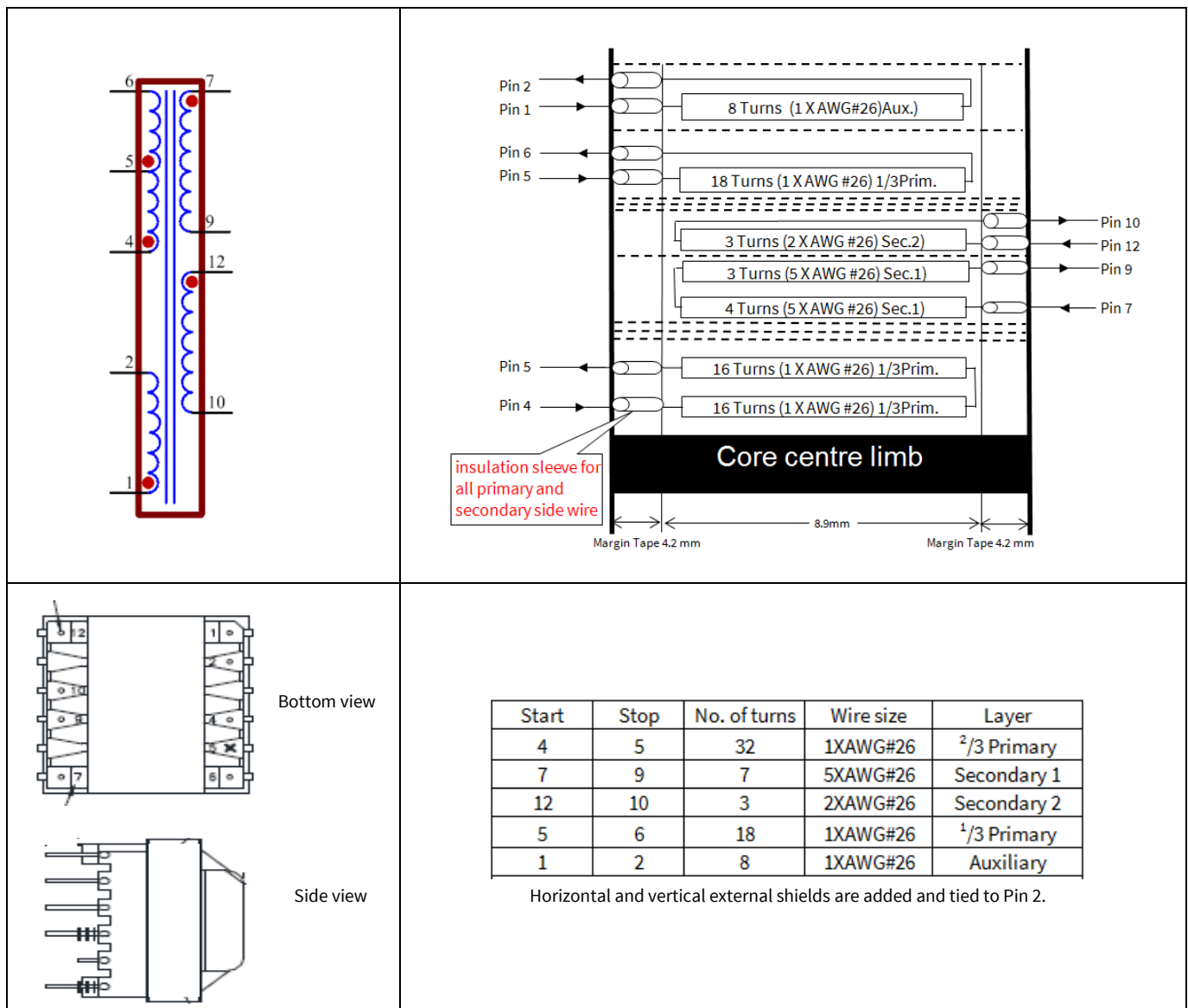
Figure 8 Transformer specifications
