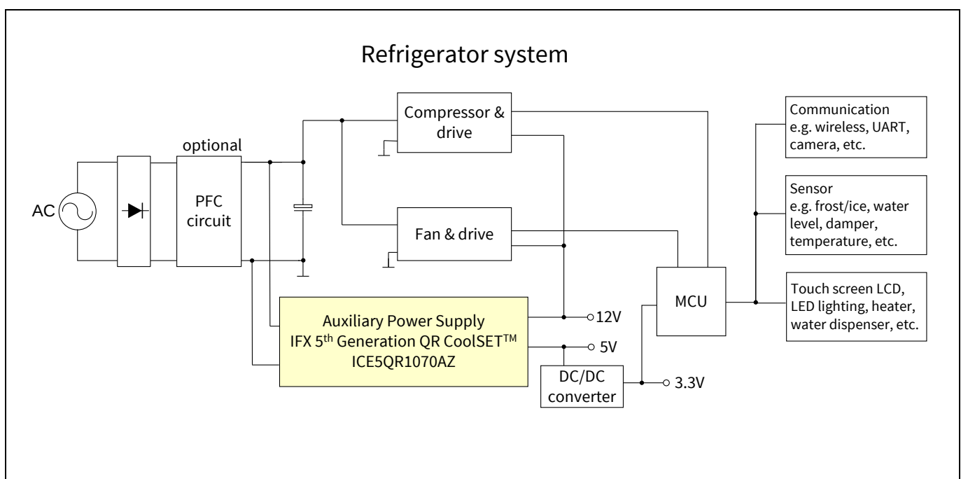
Figure 1 Simplified refrigerator system block diagram
