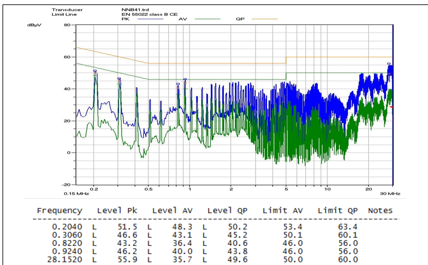
Figure 27 Conducted emissions at 230 V AC line and 33 W load - &gt; 6 dB margin
