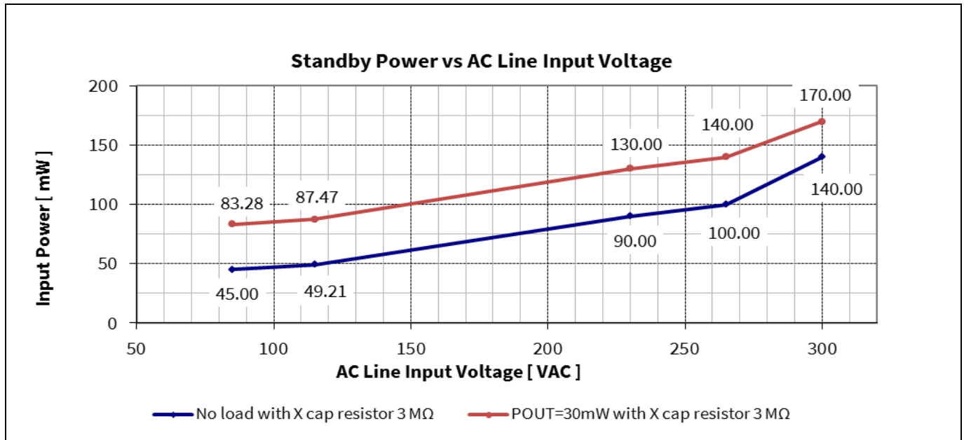
Figure 12 Standby power at no load ( P_{\text{stby\_NL}} ) and 30 mW load ( P_{\text{stby\_ML}} ) vs AC-line input voltage (measured by Yokogawa WT210 power meter – integration mode)
