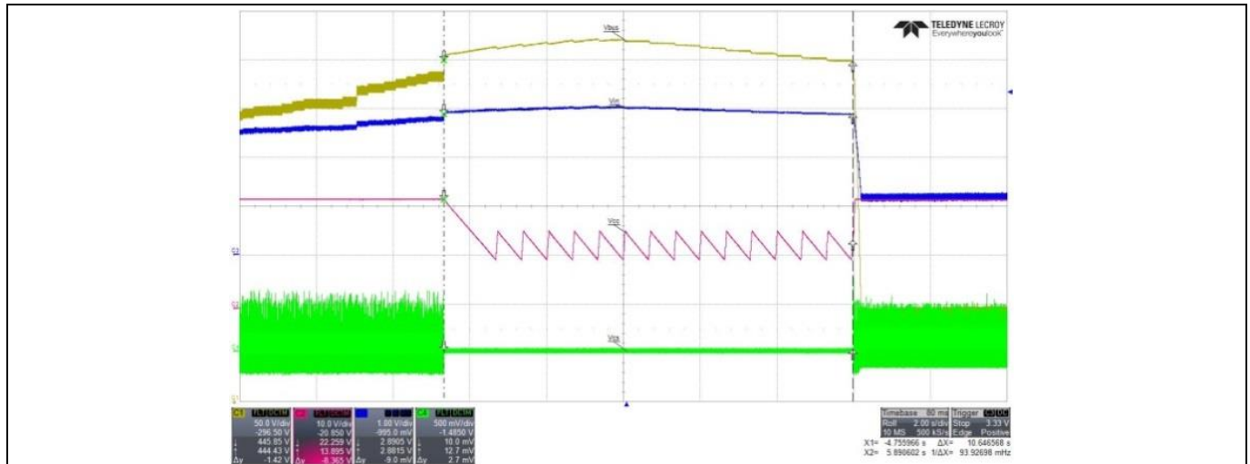
Figure 21 Line OVP
