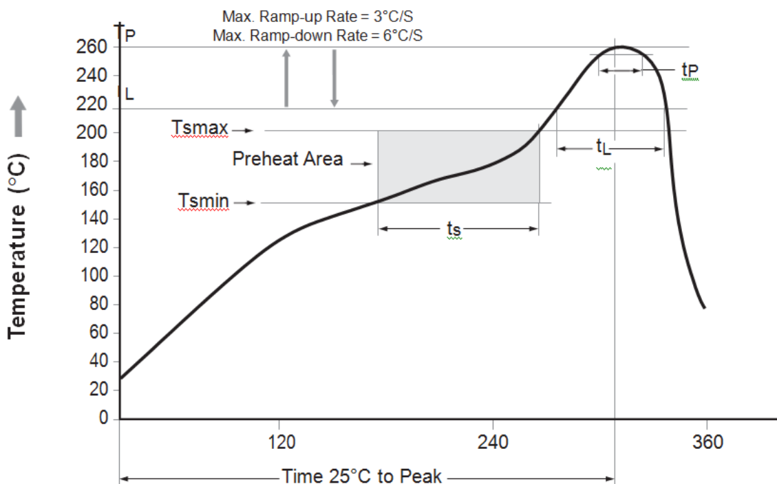
Figure 11. Reflow Profile
