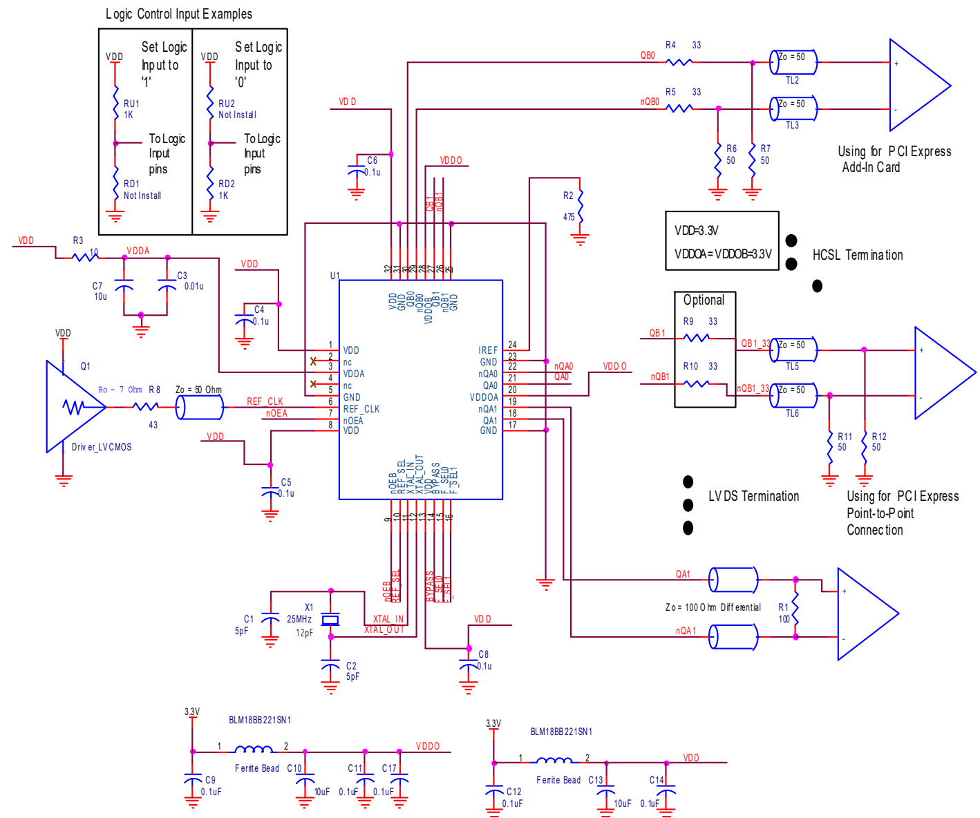
Figure 27. 841N254B Application Schematic
