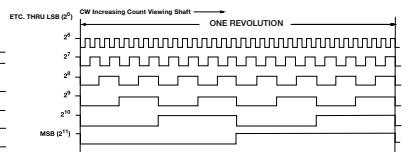
Figure 2 Natural Binary
