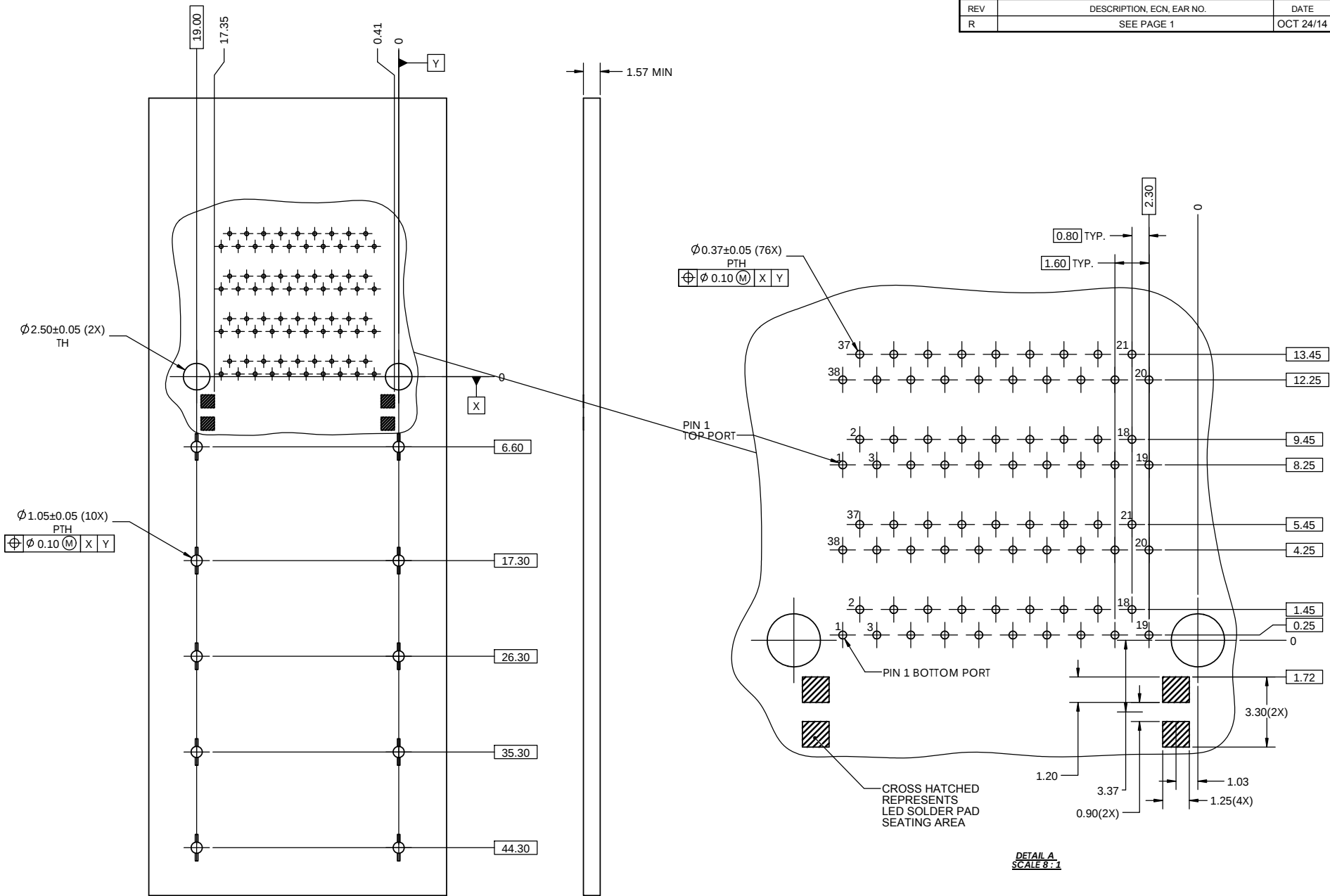
RECOMMENDED PCB BOARD LAYOUT COMPONENT SIDE SHOWN
