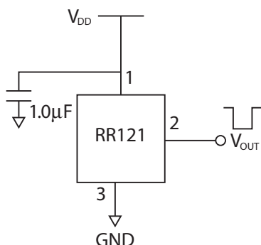
17.1 Application Circuit (SOT-23-3)
