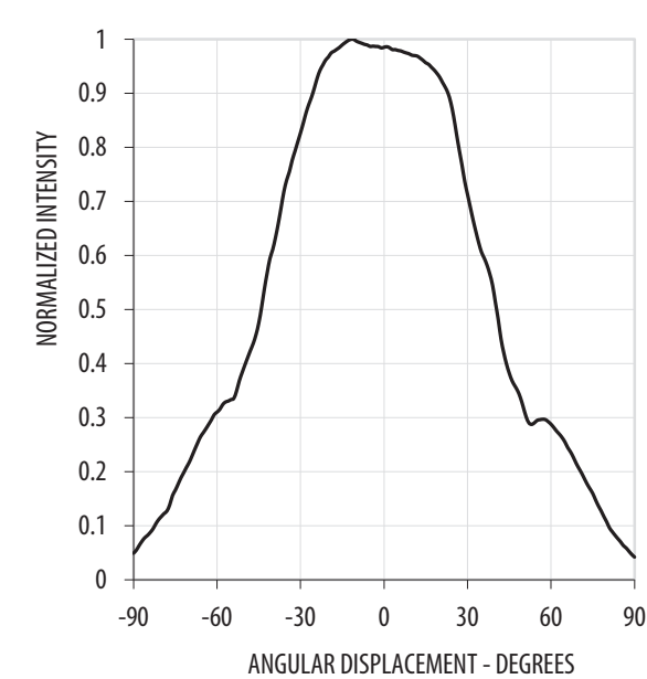
Figure 5: Radiation Pattern
