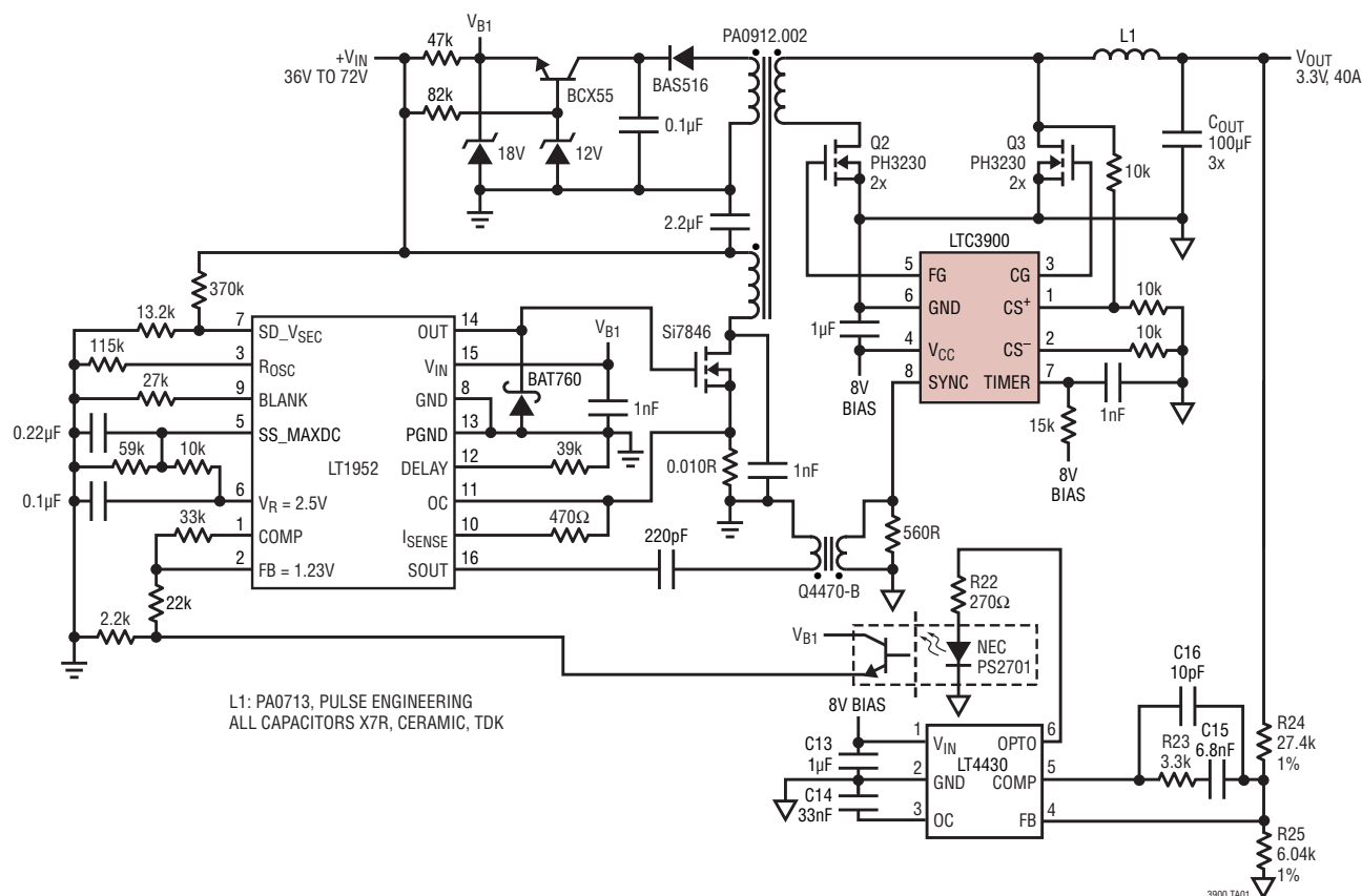
36V to 72V, 3.3V at 40A Synchronous Forward Converter
