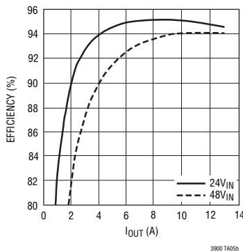
The High Efficiency of Converter is Achieved by Precise MOSFET Timing Provided by LT1952 and LTC3900 Controllers.
