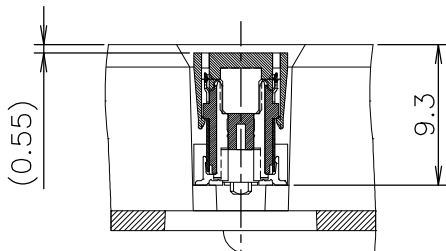
SECT. D-D (SCALE 2:1)
