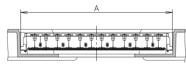
SECT. D-D (SCALE 2:1) (CONNECTOR NOT SECTION)
