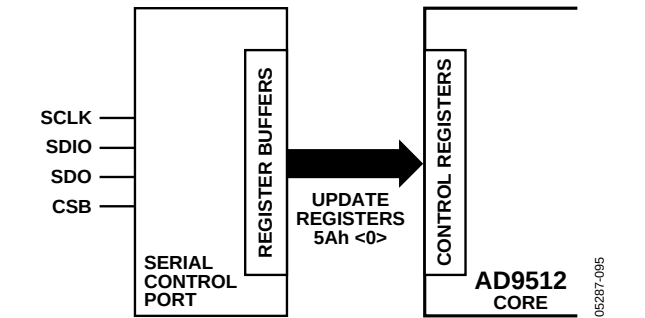
Figure 31. Relationship Between Serial Control Port Register Buffers and Control Registers of the AD9512
