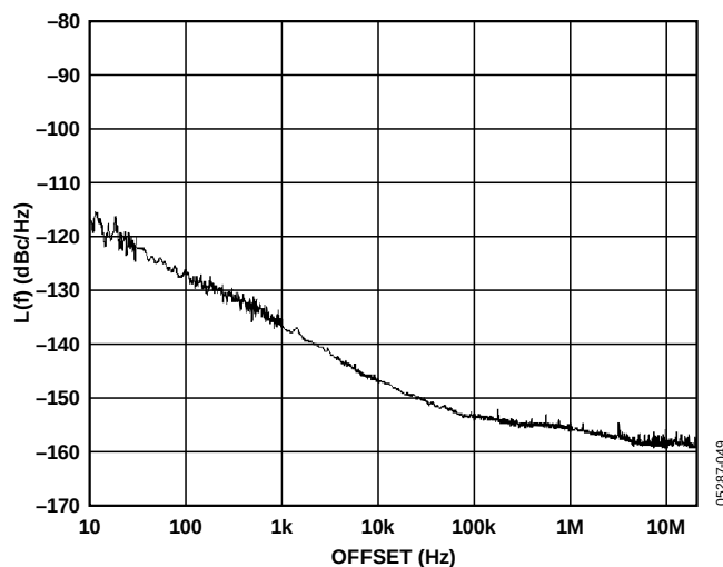
Figure 21. Additive Phase Noise—LVDS DIV2, 122.88 MHz
