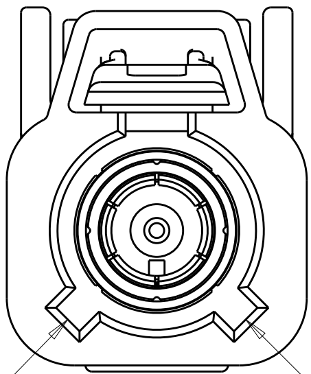
DETAIL K SCALE 5:1
