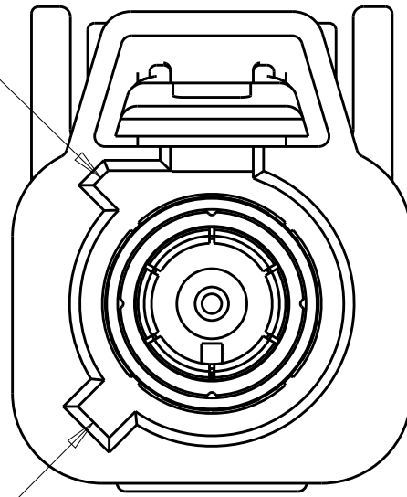
DETAIL F SCALE 5:1
