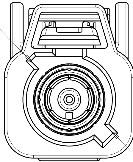
DETAIL G SCALE 5:1
