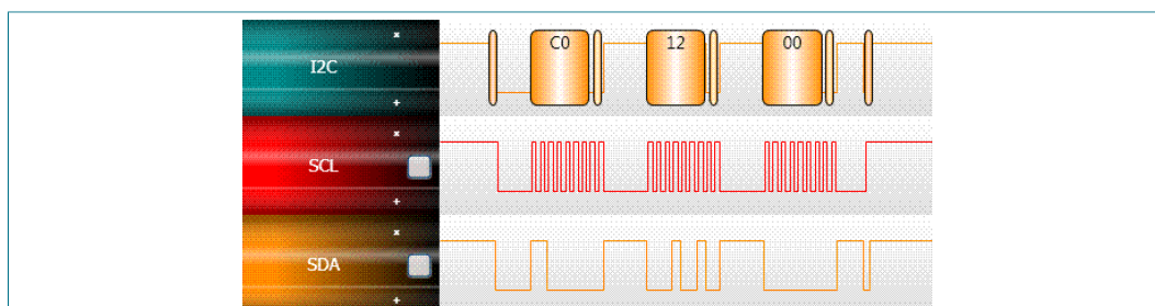
Command to I 2 C start conversion, 12h
