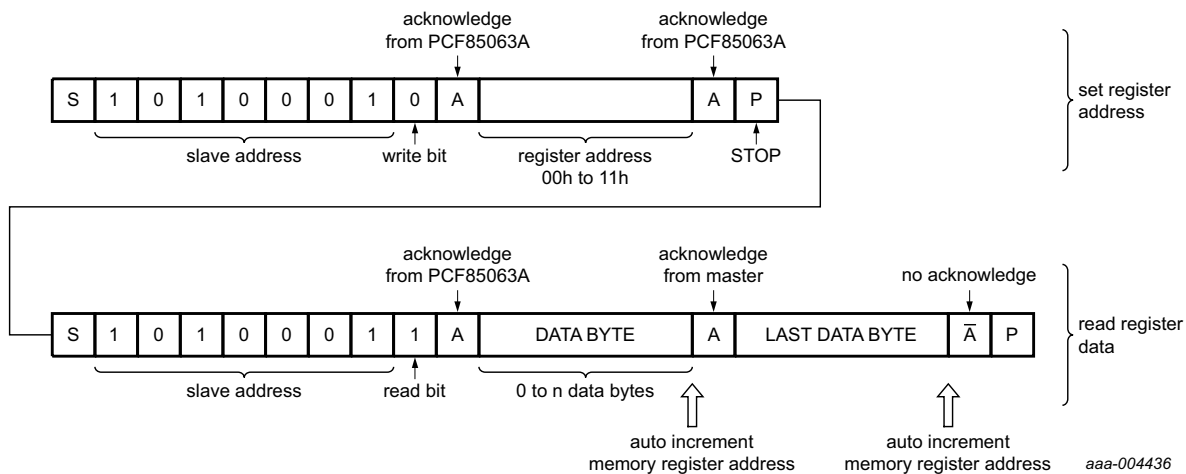
Fig 23. Master reads after setting register address (write register address; READ data)
