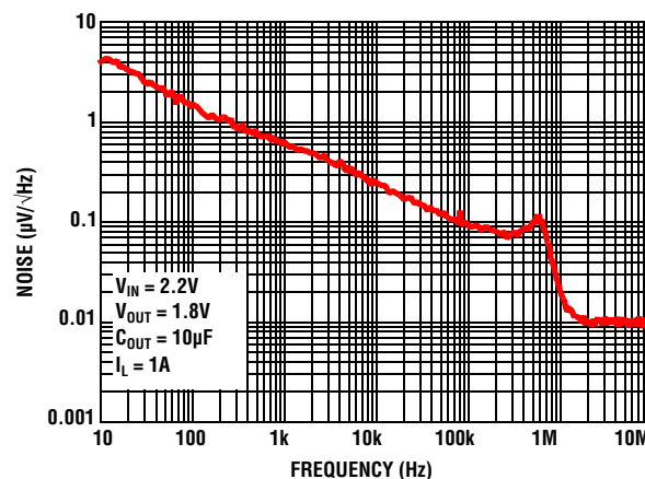
FIGURE 15. OUTPUT NOISE SPECTRAL DENSITY
