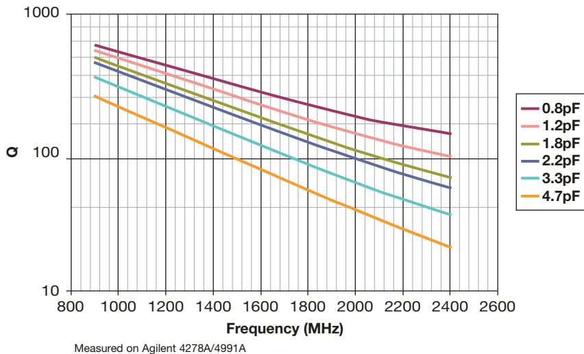
Accu-P ® 0402 Typical Q vs Frequency
