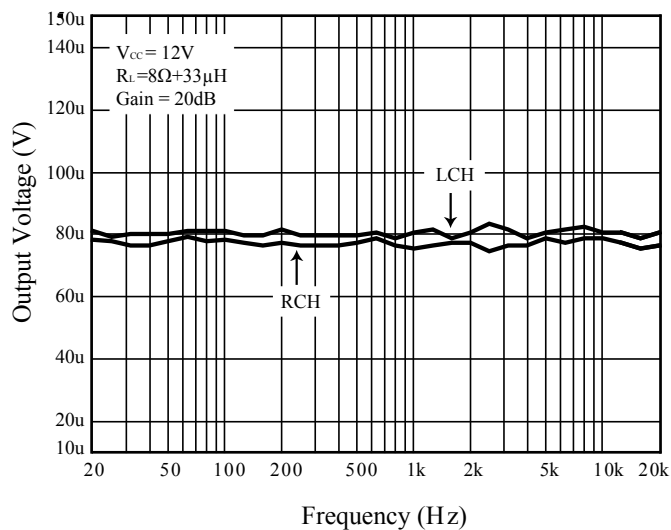
Figure 19 Noise
