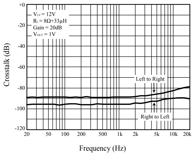
Figure 21 Crosstalk
