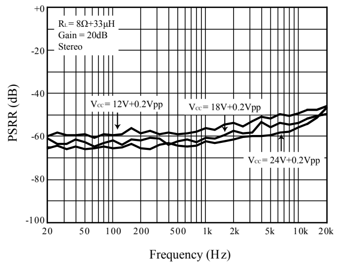
Figure 18 PSRR
