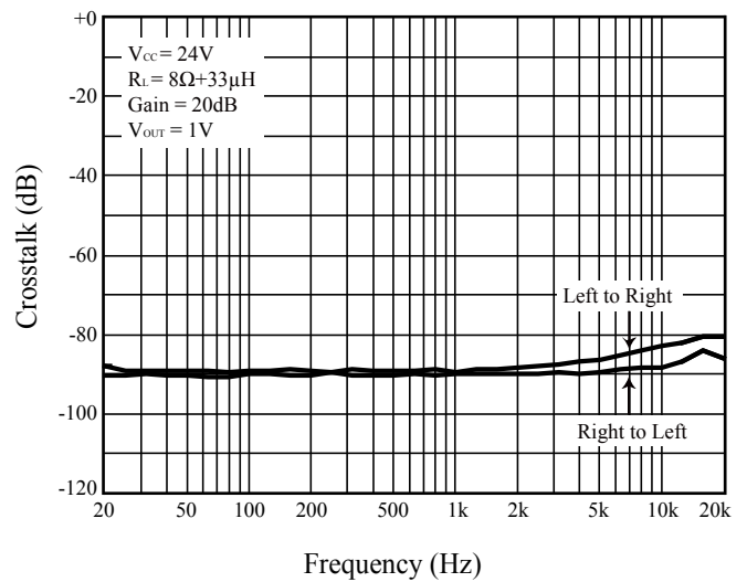
Figure 22 Crosstalk
