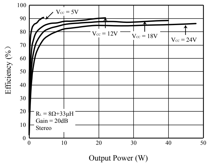
Figure 16 Efficiency vs. Output Power
