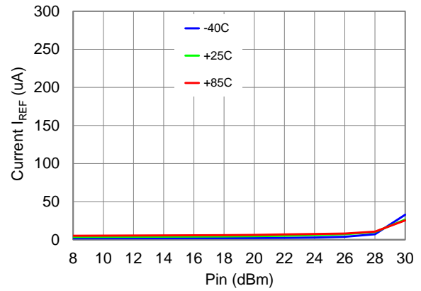
Current I_{REF} vs. Pin vs. Temperature
