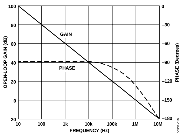
Figure 15. Open-Loop Frequency Response (A3, A4)
