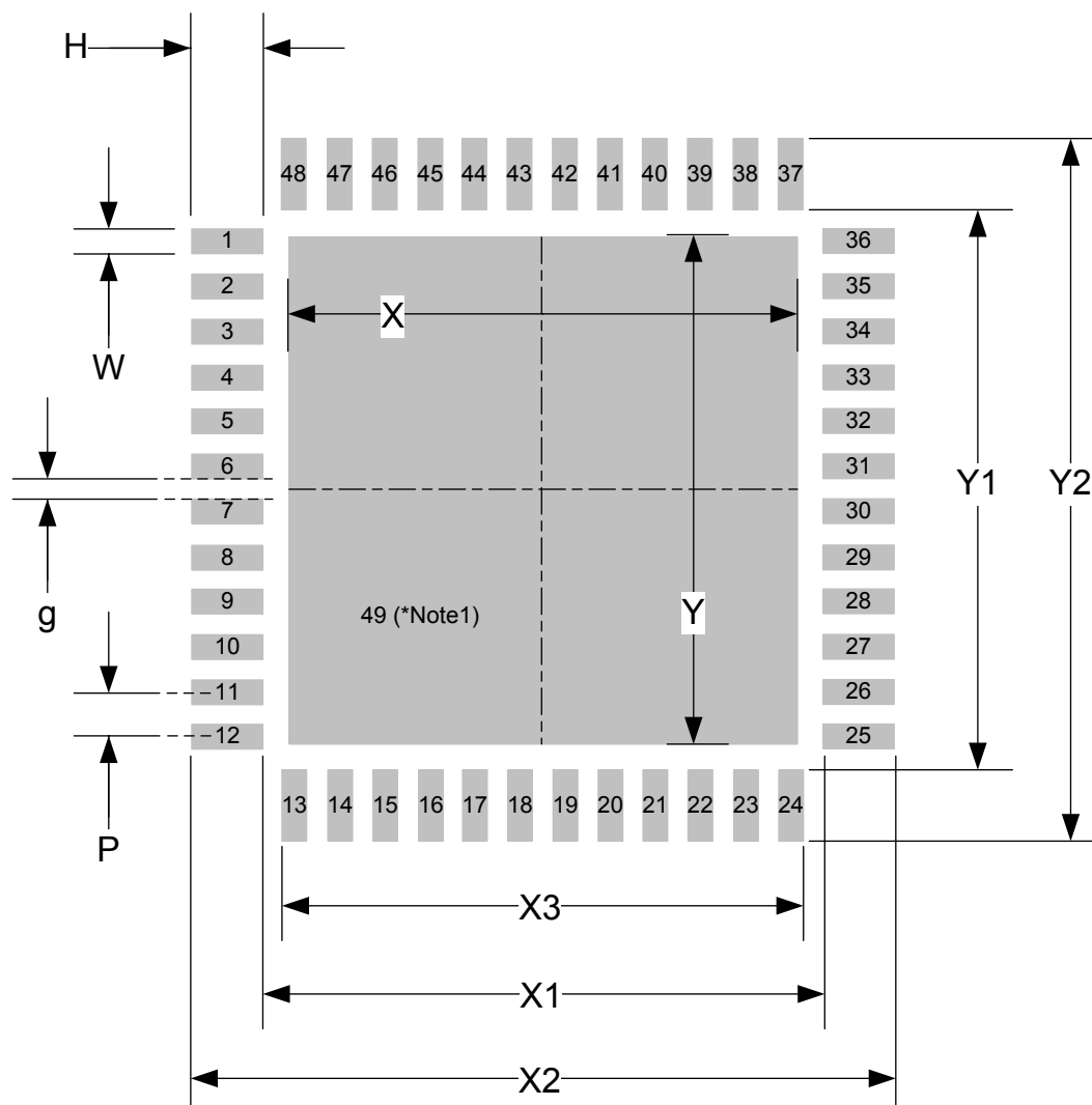
Figure 8.2 QFN(7x7)-48 Footprint
