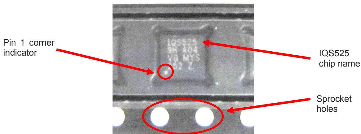
Figure 9.3 IQS525 QFN28-4x4 Package in Carrier Tape Example
