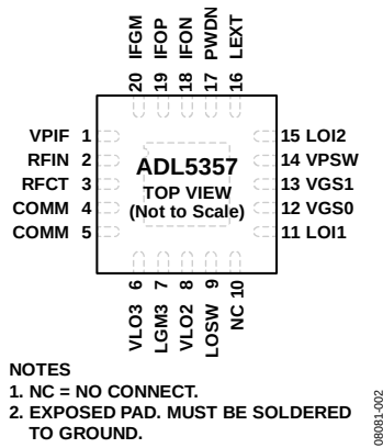
Figure 2. Pin Configuration
