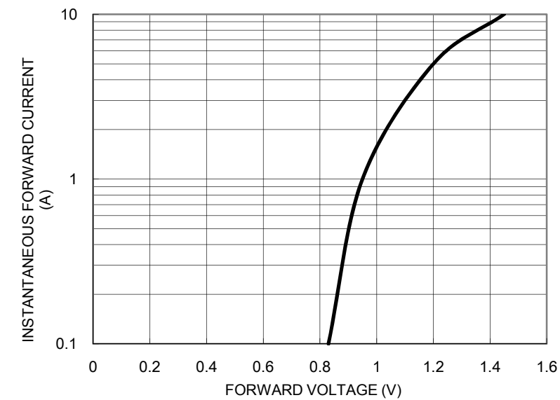
FIG. 4 TYPICAL FORWARD CHARACTERISTIC
