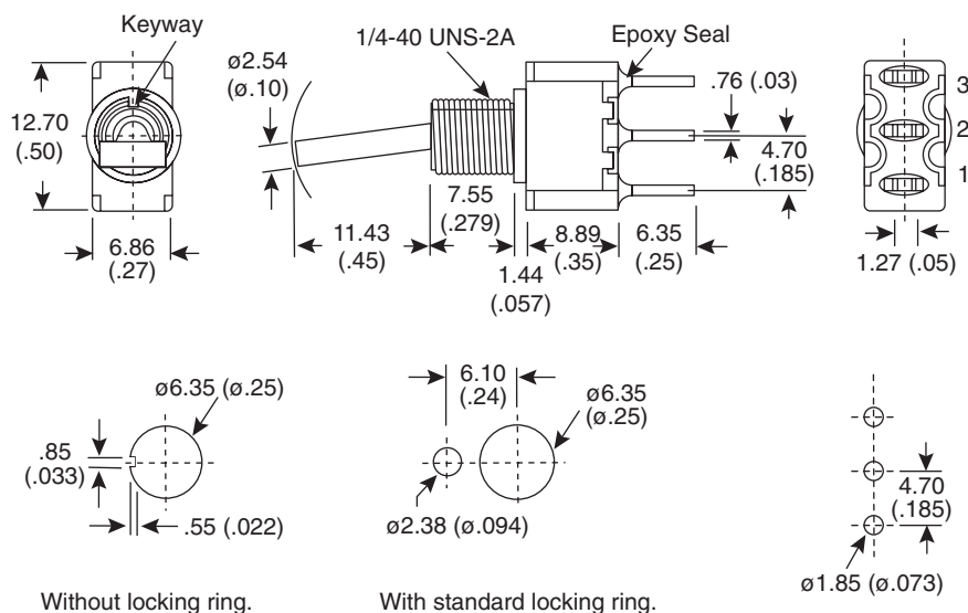
PANEL MOUNTING
