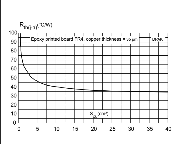
Figure 8. Thermal resistance junction to ambient versus copper surface under tab
