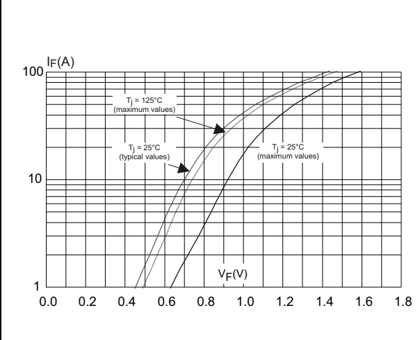
Figure 7. Forward voltage drop versus forward current (per diode)
