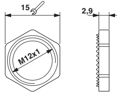
Dimensional drawing
