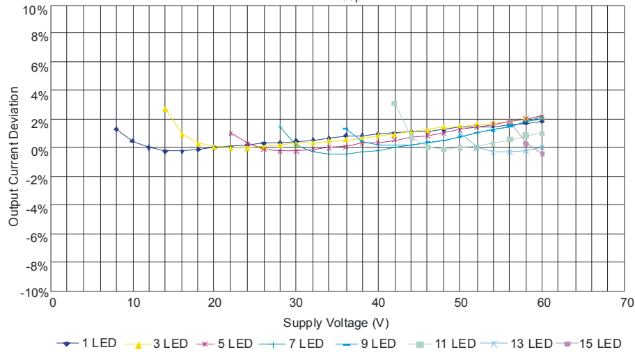
ZXLD1362 Output Current L = 150 \mu H
