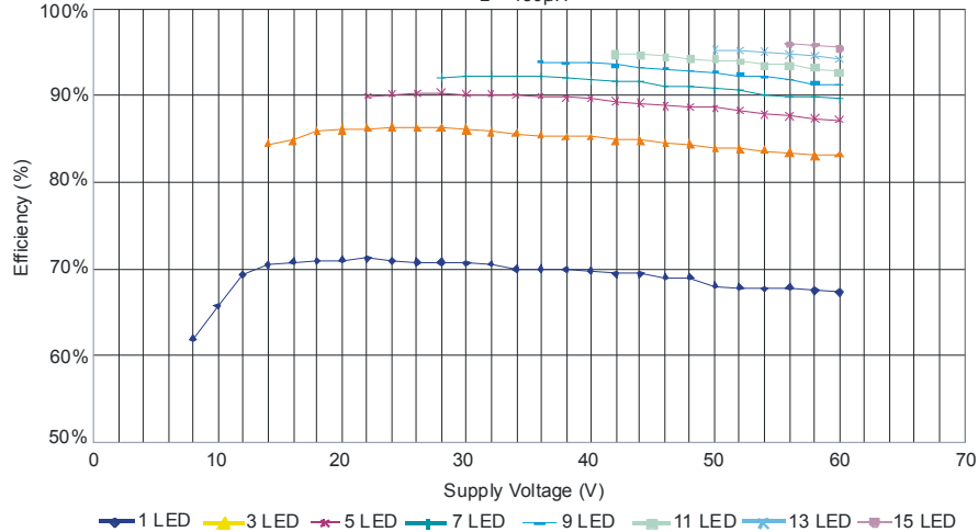
ZXLD1362 Efficiency L = 150 \mu H
