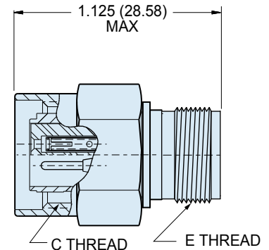
PLUG WITH ACCESSORY THREAD 802-009
