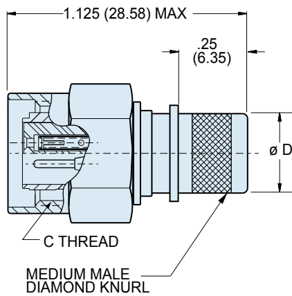
PLUG WITH INTEGRAL BAND PLATFORM 802-008
