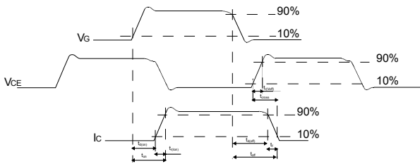
Figure 29. Switching waveform
