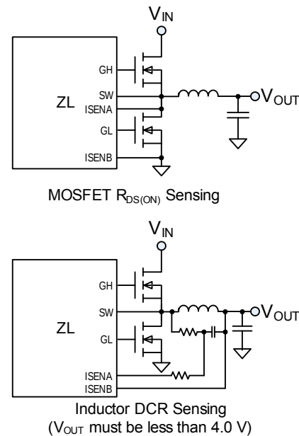
FIGURE 12. CURRENT SENSING METHODS
