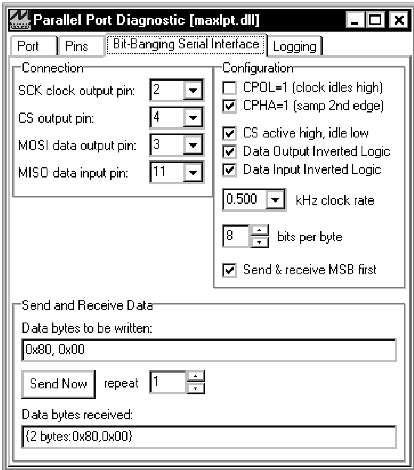
Figure 3. SPI Utility Showing the Settings to Communicate with the MAX1978 EV Kit
