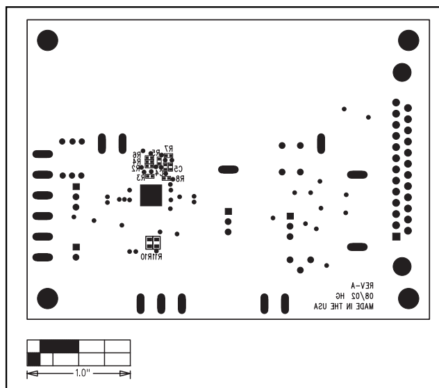
Figure 11. MAX1978 EV Kit Component Placement Guide (2oz Copper)—Solder Side
