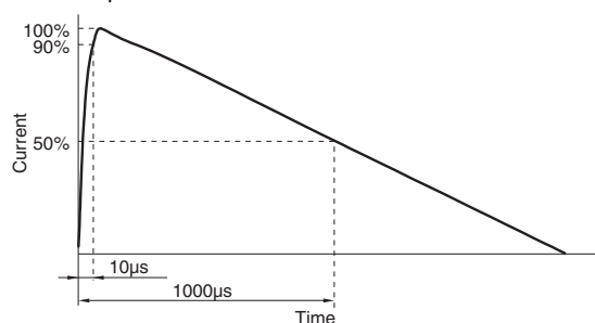
* 2 10/1000μs test waveform
