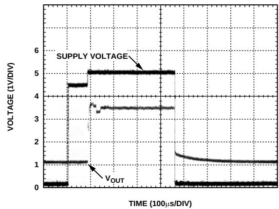
Figure 33. Power-On Response at 125^{\circ}C
