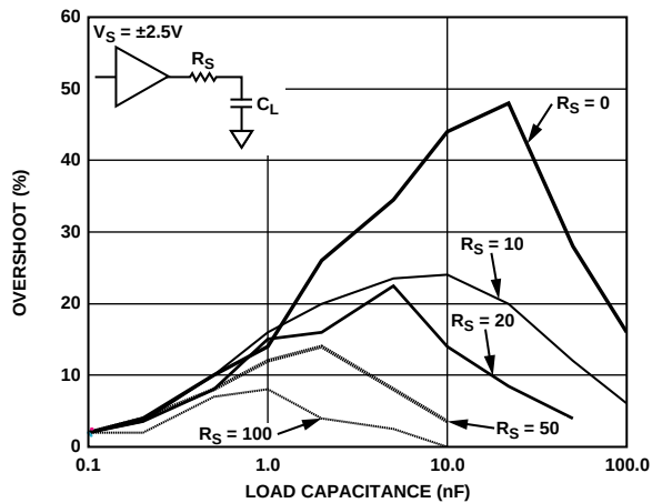
Figure 58. Negative Overshoot Graph vs. C_L
