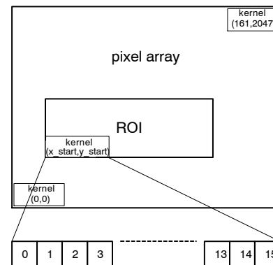
Figure 37. Kernel Organization in Pixel Array
