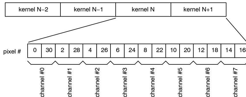
Figure 42. Data Output Order for 8 LVDS Output Channels in Subsampling Mode on a Monochrome Sensor
