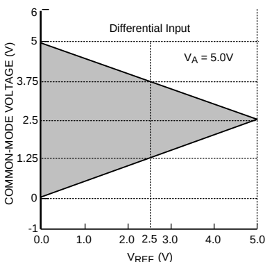
Figure 36. V_{CM} range for Differential Input operation
