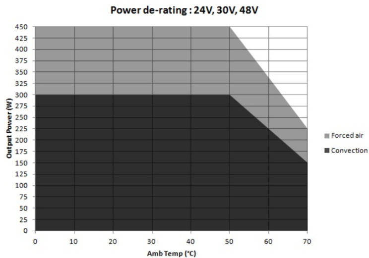
Figure 1. Derating Curves
